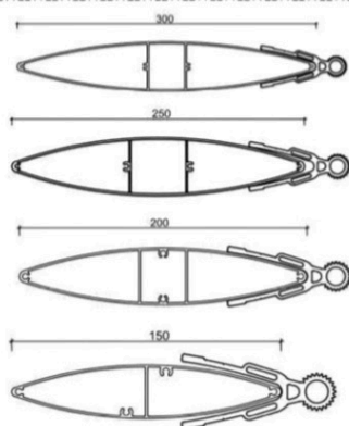
Other System - Sun Shading
